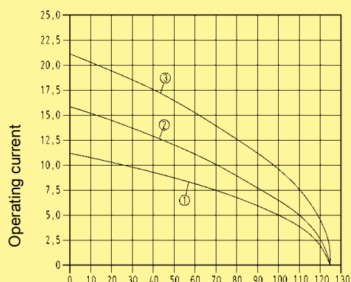
Ambient temperature
