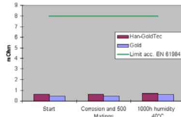
Contact resistance Gold - GoldTec Han ® D contacts
